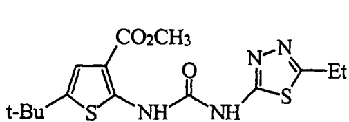
5 5-tert-Butyl-2-(3-(5-ethyl-[1,3,4]thiadiazol-2-yl)-ureido)-thiophene-3-carboxylic acid methyl ester
